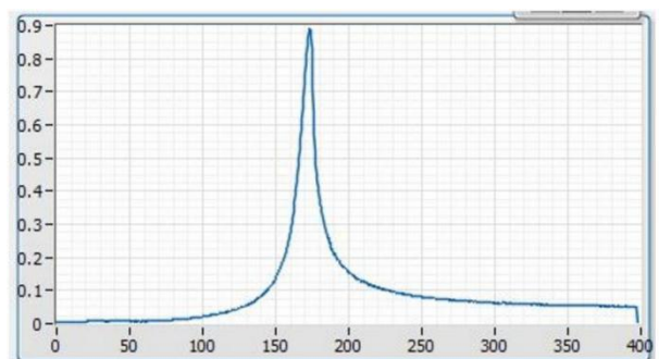
Figure 2. Acceleration-over-frequency chart from 0 ~ 400Hz
