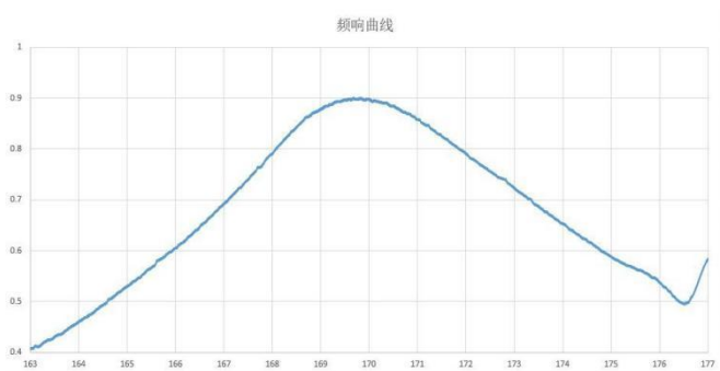
Figure 1. Linear Vibrator Frequency Characteristics/频率特性
